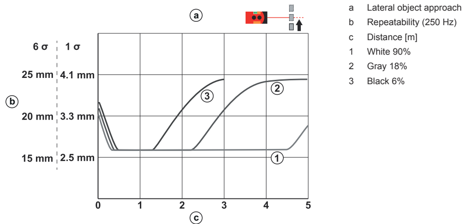
Repeatability (250 Hz)
