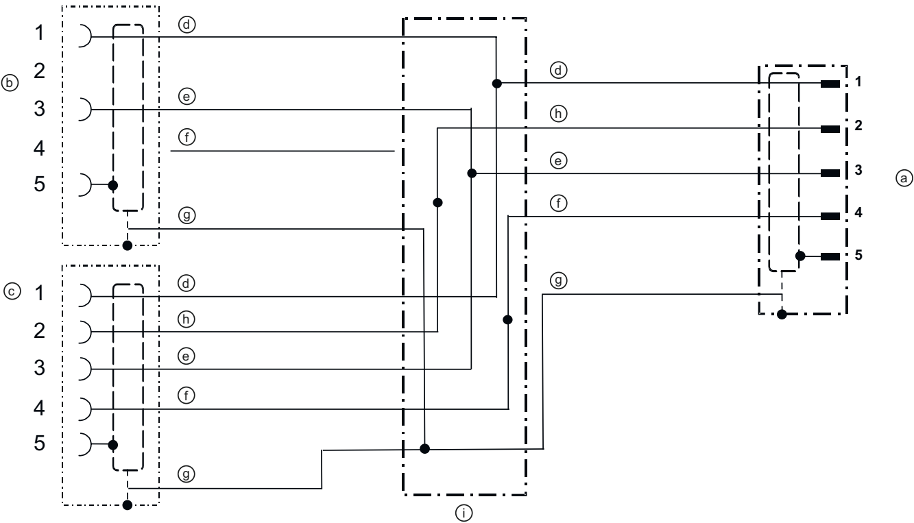
Connection diagram
