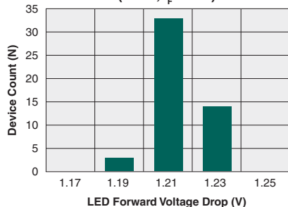
Typical LED Forward Voltage Drop (N=50, I_F=8\text{mA} )
