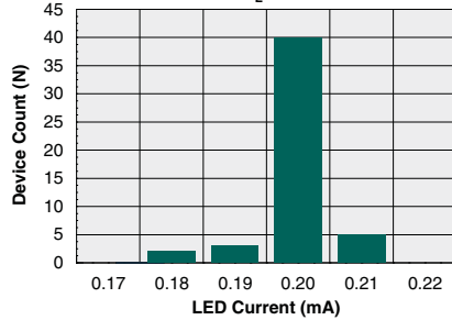
Typical I_F for Switch Operation (N=50, I_L=150\text{mA} )
