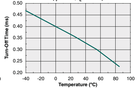
Typical Turn-Off Time vs. Temperature ( I_F=5\text{mA} , I_L=80\text{mA} )
