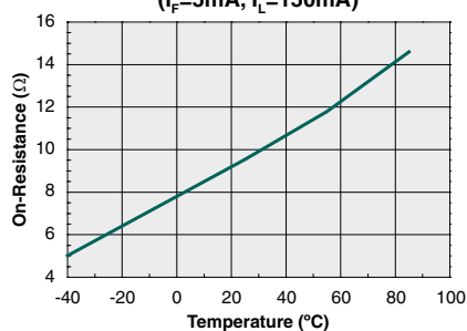
Typical On-Resistance vs. Temperature ( I_F=5\text{mA} , I_L=150\text{mA} )
