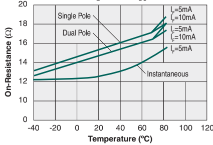
Typical On-Resistance vs. Temperature ( I_L=170\text{mA}_{DC} )
