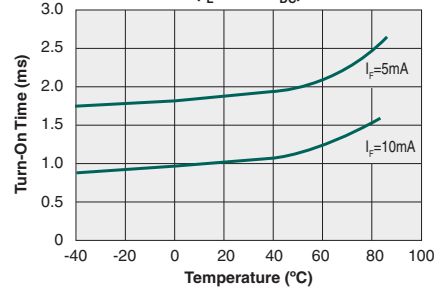
Typical Turn-On Time vs. Temperature ( I_L=80\text{mA}_{DC} )
