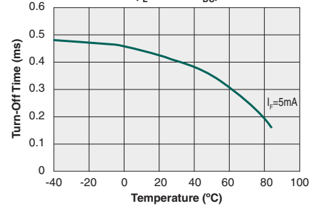
Typical Turn-Off Time vs. Temperature ( I_L=120\text{mA}_{DC} )
