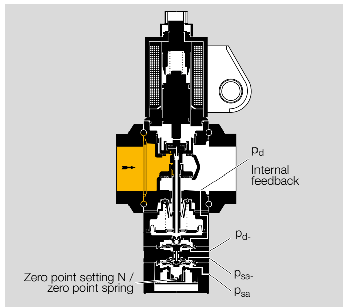
VAH (VRH: no valve)
