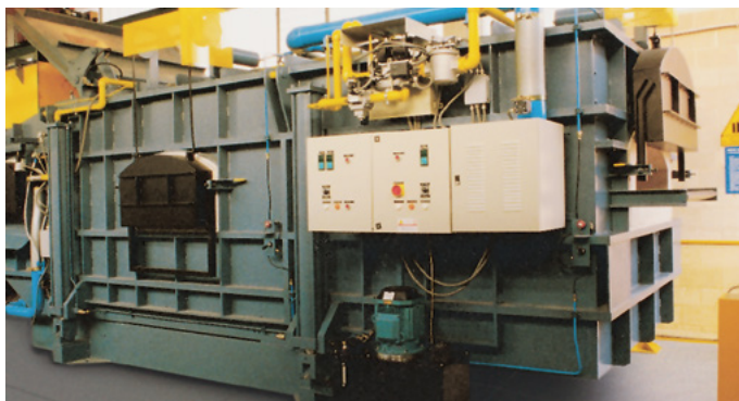
Air/gas ratio control on melting furnace for ensuring stoichiometric combustion over the entire capacity range
