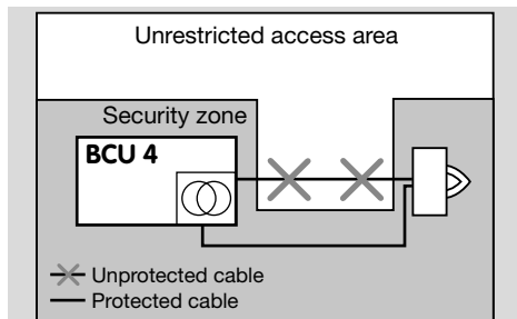
Protected and unprotected wiring
