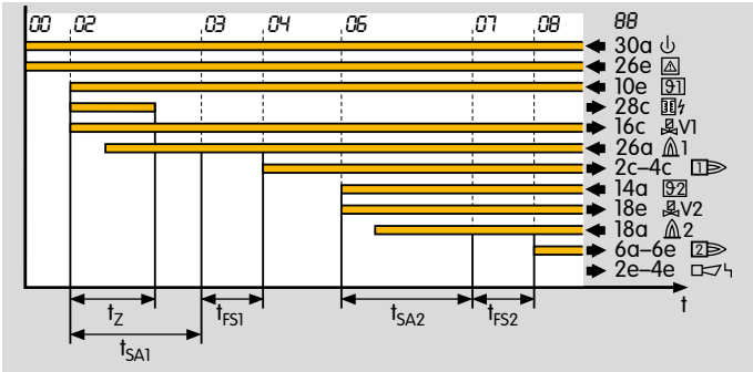
Safety time on start-up t_{SA2} for the main burner.
