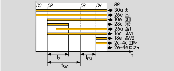
Safety time on start-up t_{SA1} for the pilot burner.
