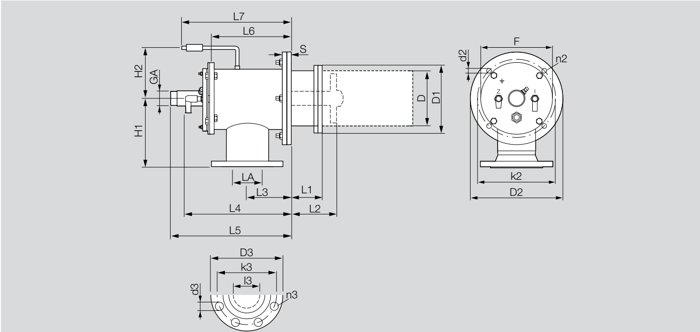
ZICW Standard: L1 = 100, 200, 300, 400 mm and L2 = L1 + 35 mm, see page 17 (Burner length for horizontal installation)
