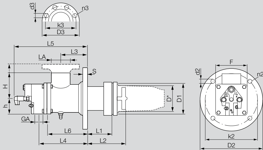
BIC Standard: L1 = 100, 200, 300, 400 mm and L2 = L1 + 35 mm, see page 17 (Burner length for horizontal installation)
