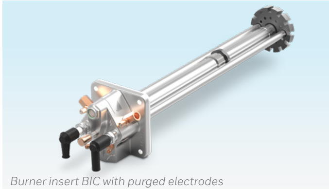
Burner insert BIC with purged electrodes
