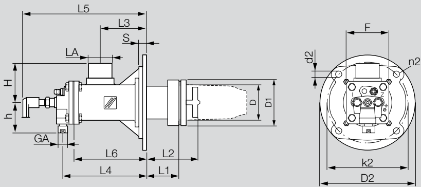
BICA Standard: L1 = 100, 200, 300, 400 mm and L2 = L1 + 35 mm, see page 17 (Burner length for horizontal installation)
