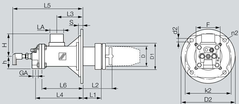
BICA Standard: L1 = 100, 200, 300, 400 mm and L2 = L1 + 35 mm, see page 17 (Burner length for horizontal installation)
