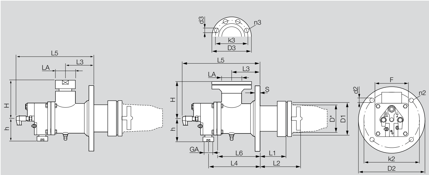
BIC Standard: L1 = 100, 200, 300, 400 mm and L2 = L1 + 35 mm, see page 17 (Burner length for horizontal installation)
