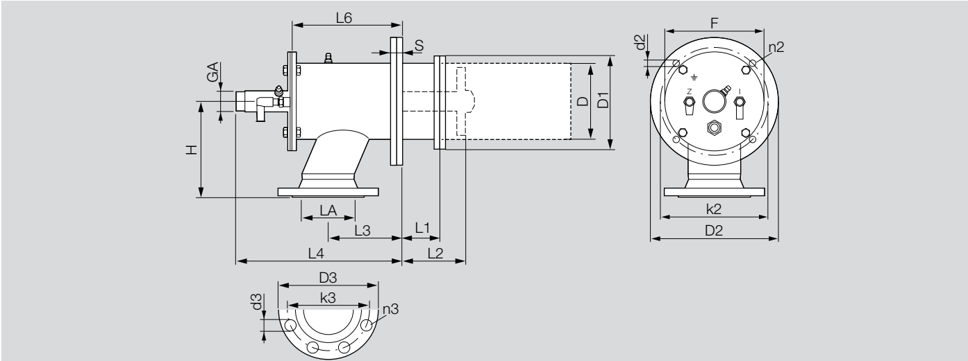
ZIC Standard: L1 = 100, 200, 300, 400 mm and L2 = L1 + 35 mm, see page 17 (Burner length for horizontal installation)
