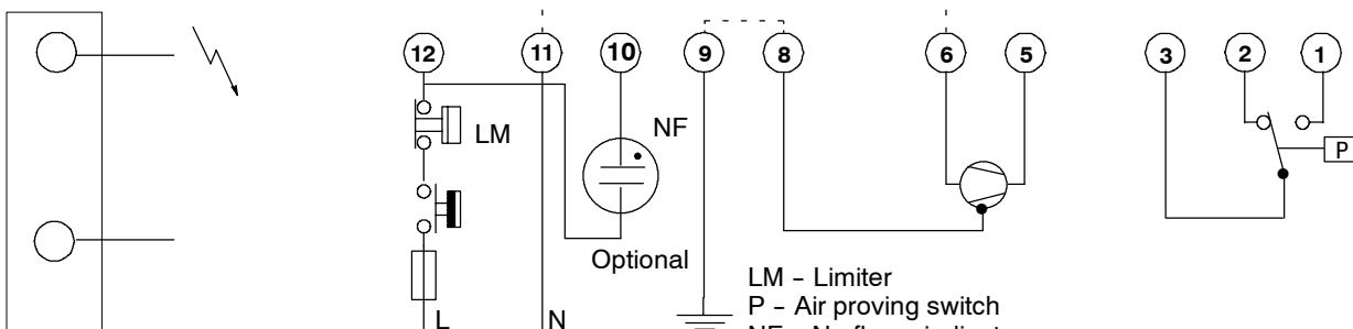
Fig. 45. Connection diagram S4585D wired up in atmospheric application
