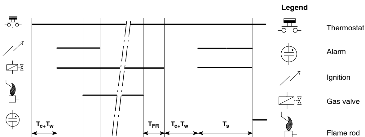
Fig. 4. Functional diagram S4565A, B, P, Q
