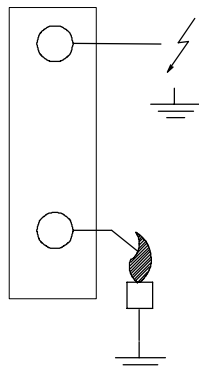
Fig. 28. Alternative side connection if sparking to ground
