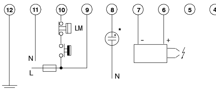
Fig. 13. Connection diagram S4565QD with external ignition circuit
