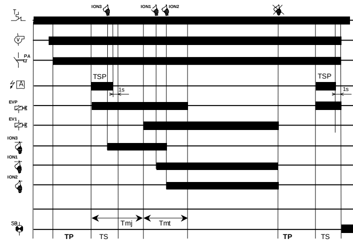
TGRD WITH OPTIONS RE3 MJnn MTnn Wnn
