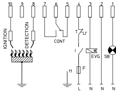
TYPE SM191N
