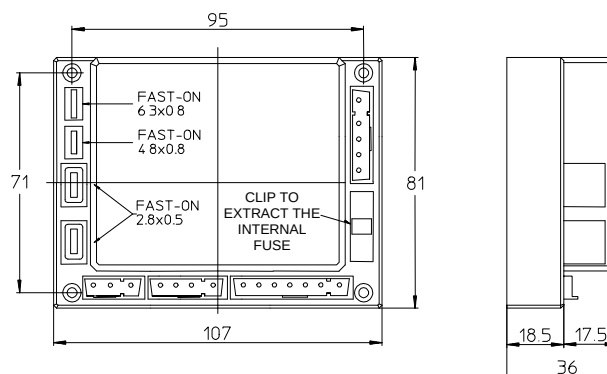
Fig. 1 – Overall dimensions
