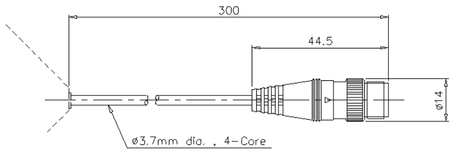
Detail of cable + connector
