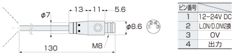
pz_m72p_dimension_02.gif
