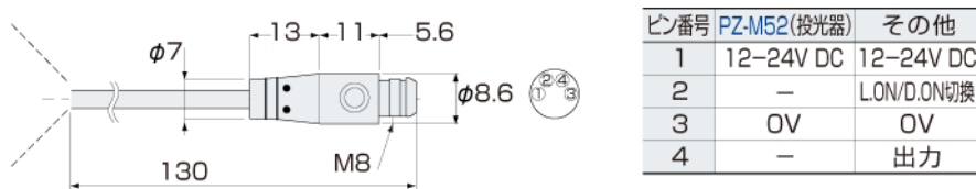
pz_m52p_dimension_02.gif
