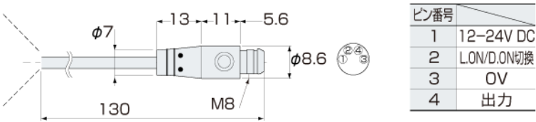
pz_m12_dimension_02.gif
