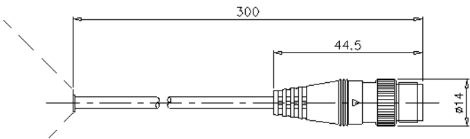
Detail of cable + connector
