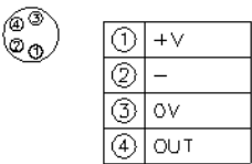
Pin arrangement
