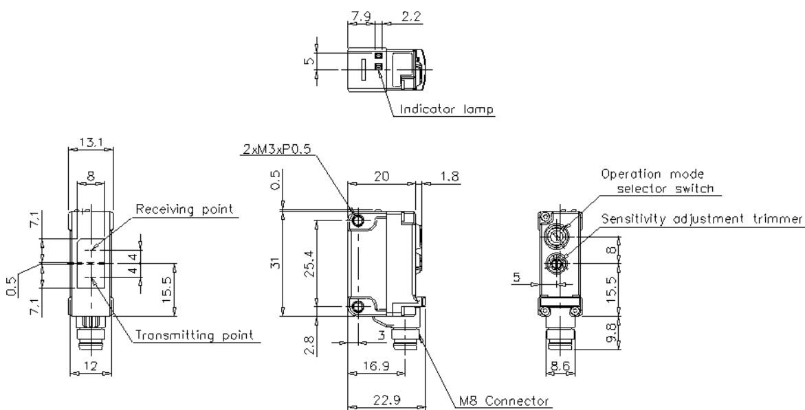
Pin arrangement
