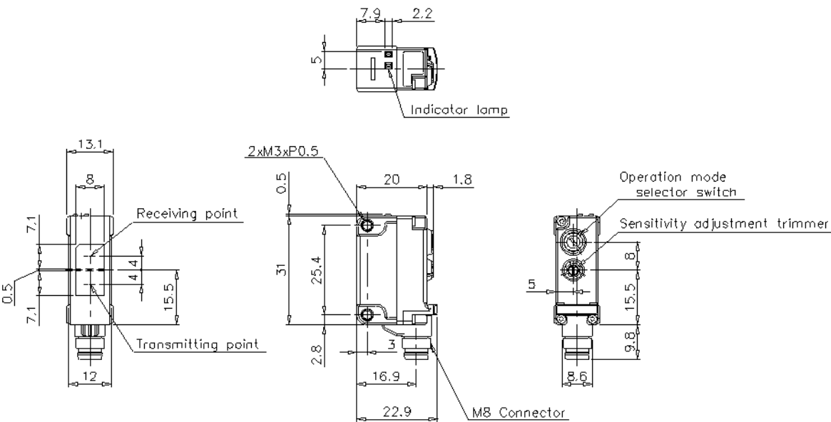
Pin arrangement
