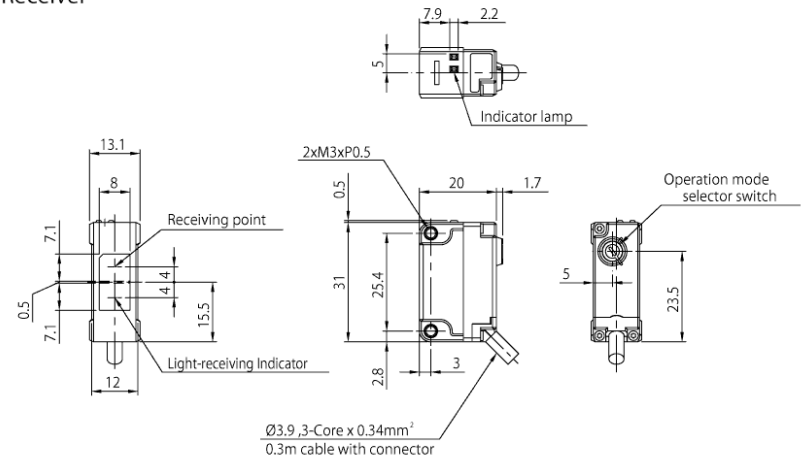
Transmitter
