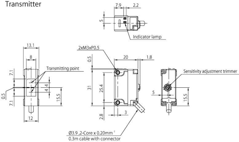
Detail of cable + connector
