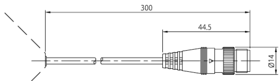
Detail of cable + connector
