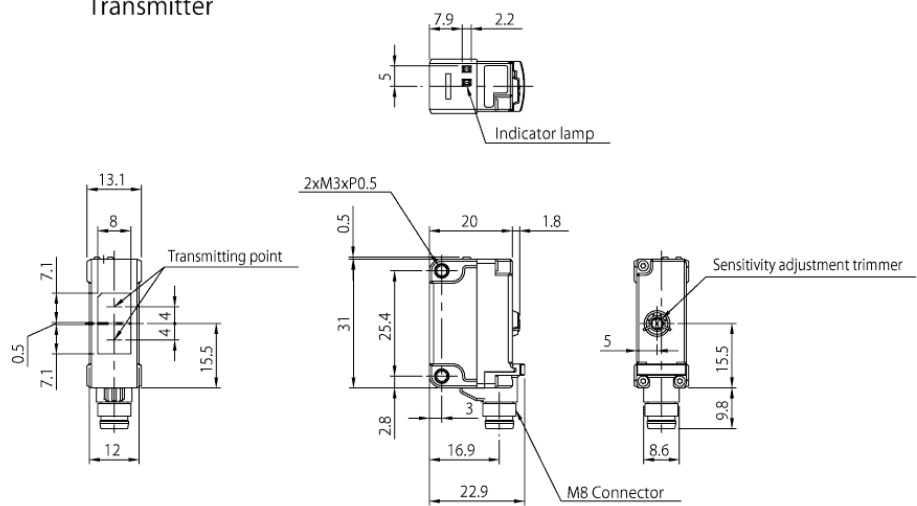
Pin arrangement
