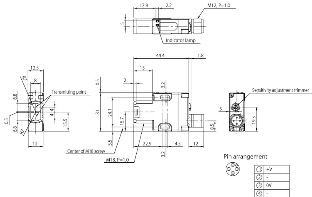
Transmitter
