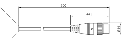
Detail of cable + connector
