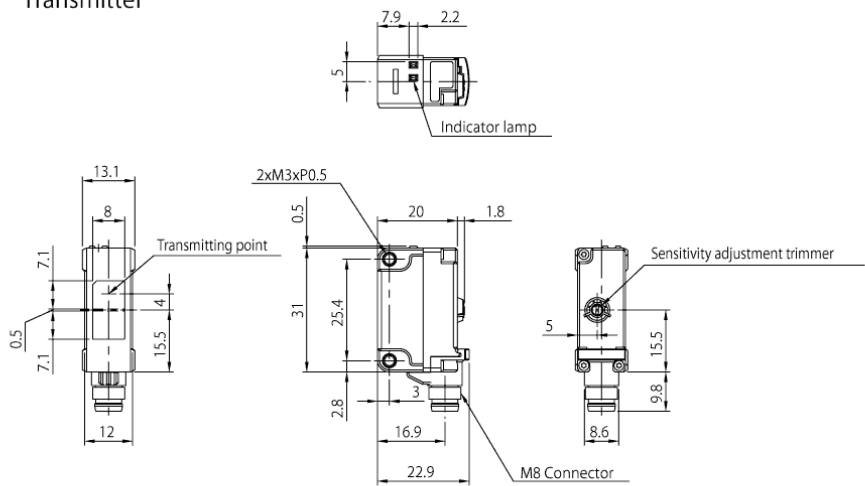
Transmitter
