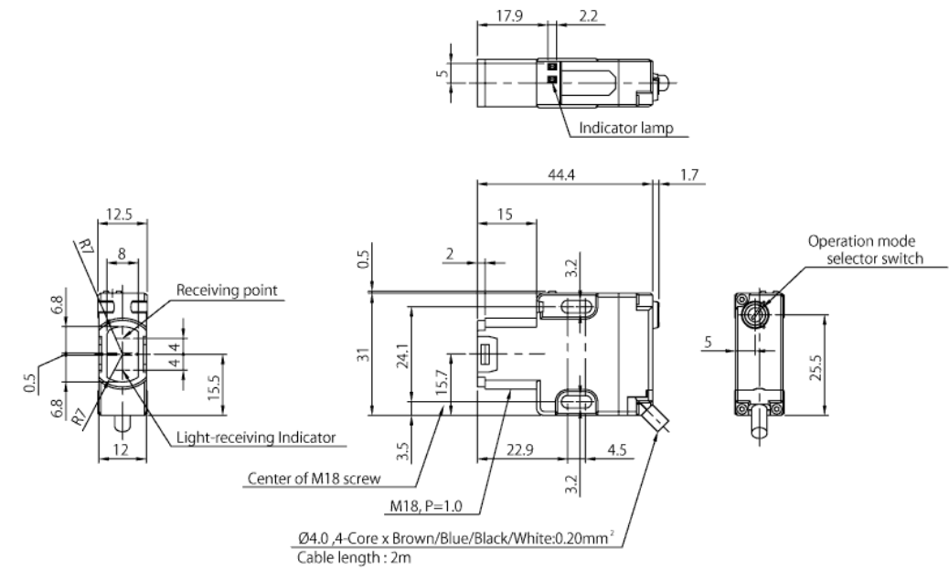
Receiver
