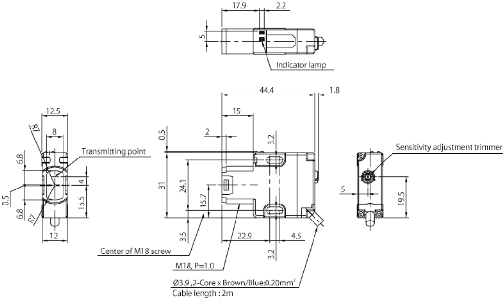
Transmitter
