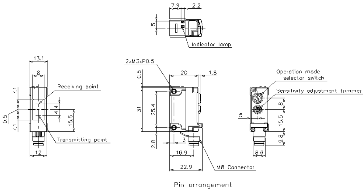
Pin arrangement
