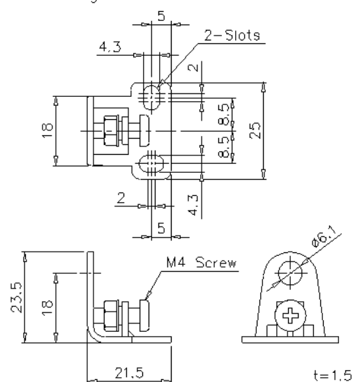
Mounting bracket
