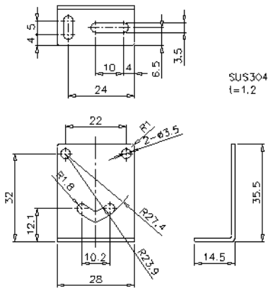
Mounting bracket
