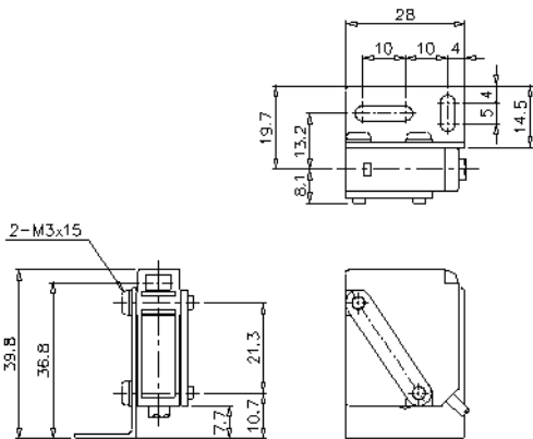
When mounting bracket is attached
