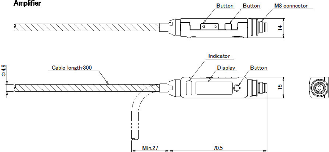
Amplifier
