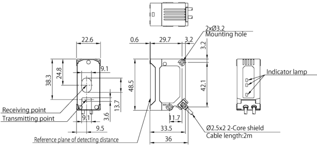
Insulating sheet(Accessory)
