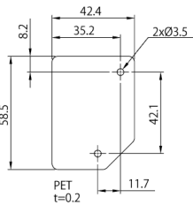
Mounting bracket(Accessory)
