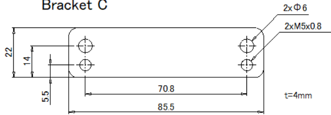
Bracket C
