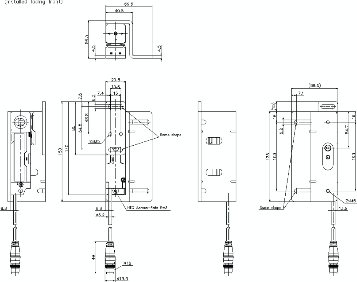
Sensor + Actuator (Installed facing front)
