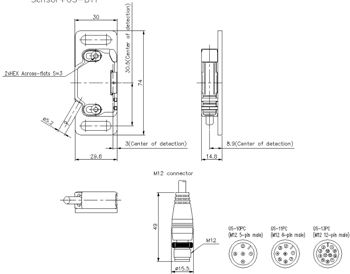
Sensor+GS-B11
