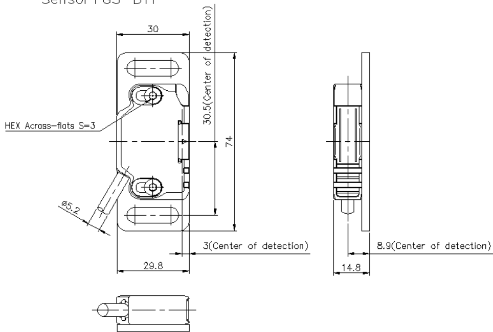
Sensor+GS-B11
