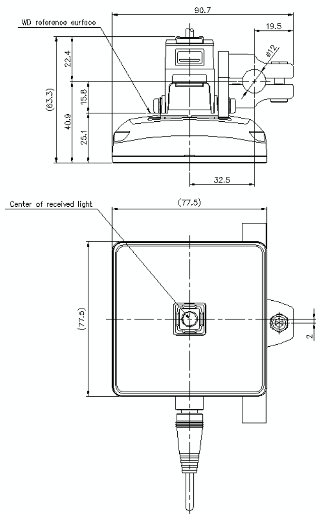
aib_d32b_88116_dimension_01.gif
