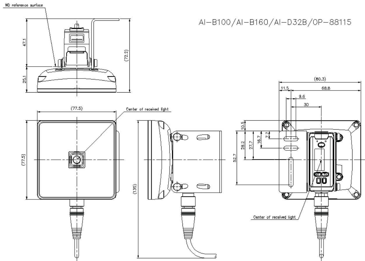
aib_d32b_88115_dimension_01.gif
