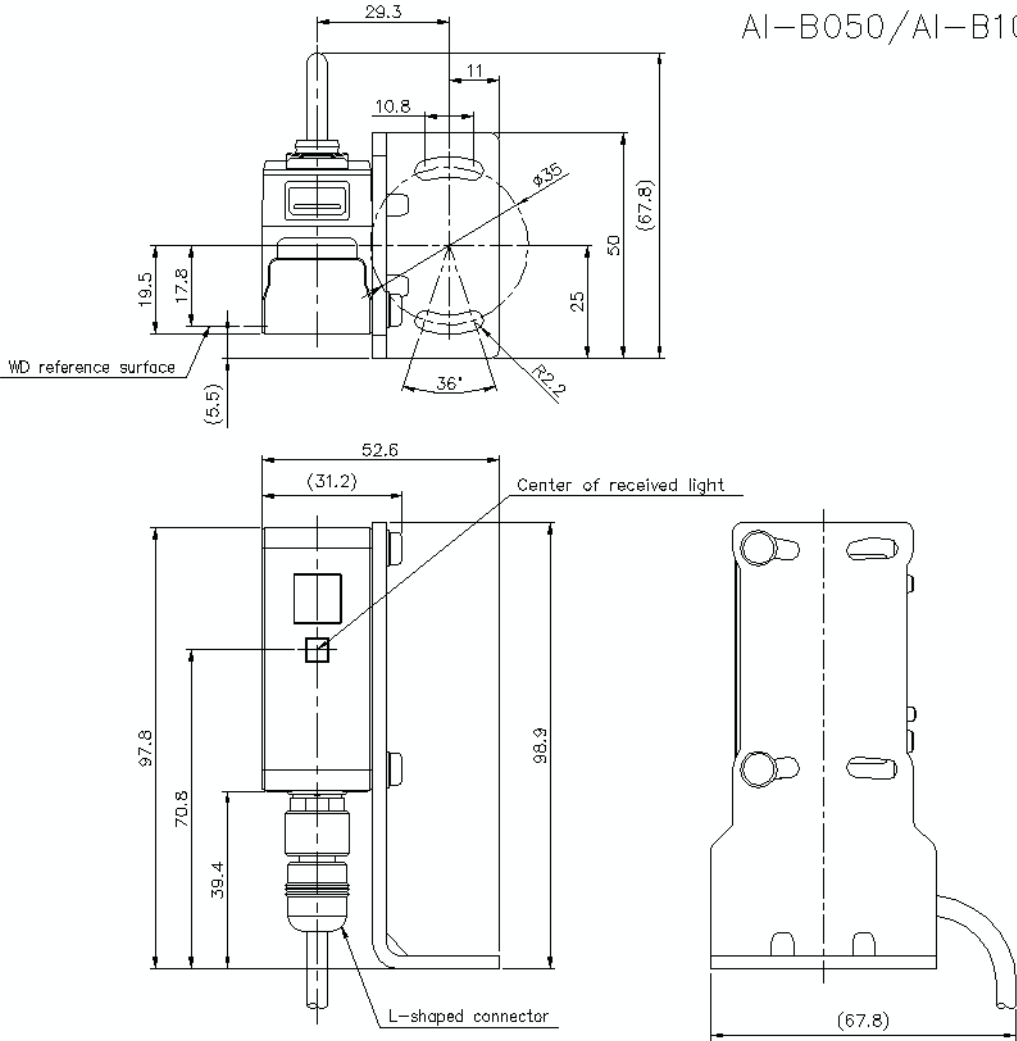
aib050_100_88114_dimension_01.gif
