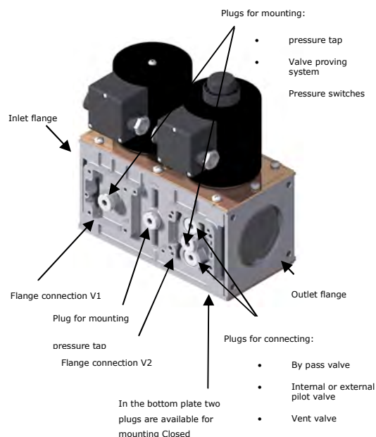
Figure 3 Interfaces for possible accessories
