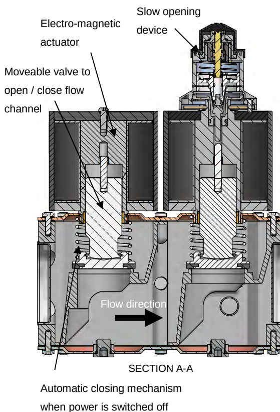
Figure 14 Schematic drawing of VQ400M.
