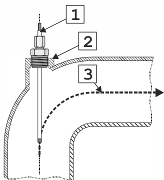
Fig. 2. ≤ DN50, elbow pipe
