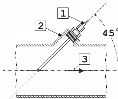
Fig. 3. ≤ DN50, straight pipe
