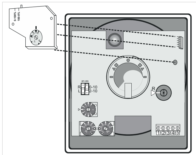
Fig. 2 Mounting VMU1
