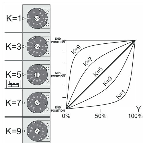
Fig. 7 Characteristic curve
