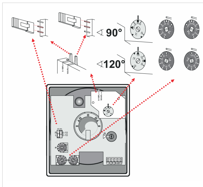
Fig. 3 Adjusting settings
