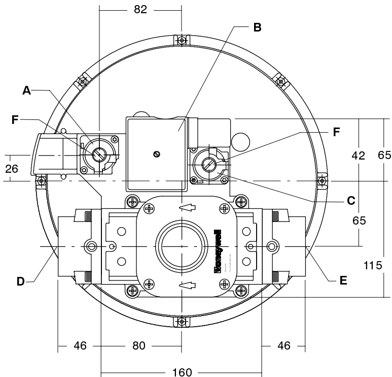
Fig. 2. V4085 (1 1/2" and 2")
