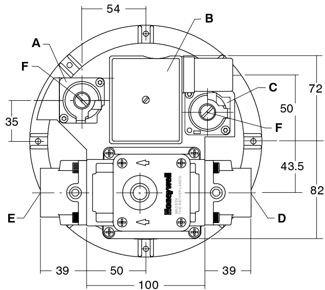
Fig. 1. V4085 (3/4" and 1")
