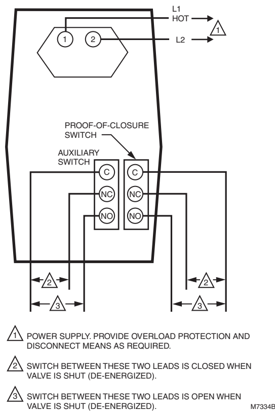
Fig. 4. External connections to the V4055 Actuator.
