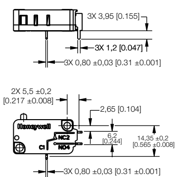
Figure 14. V15 Series L-style Left-Side PCB Terminal
