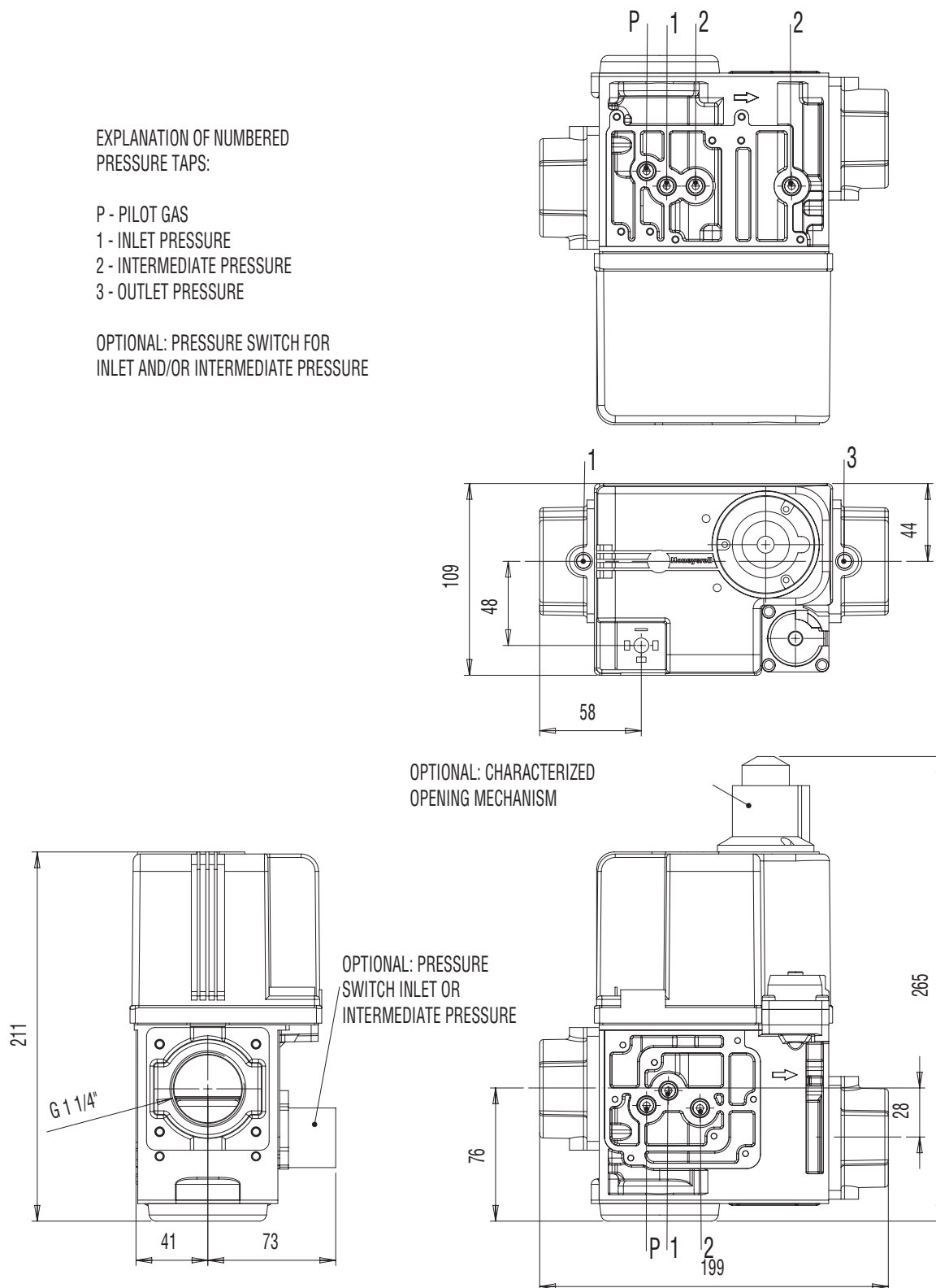
Fig. 6a. Dimensional drawing VR434/VR834 series (DN32)
