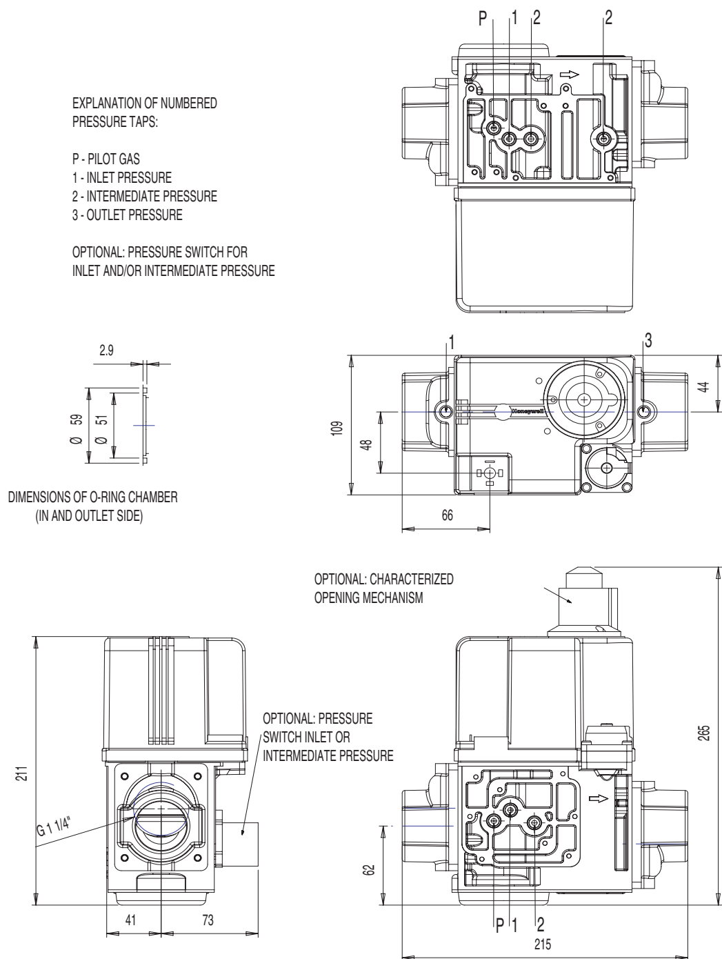
Fig. 7. Dimensional drawing VR434/VR934 series (DN34)
