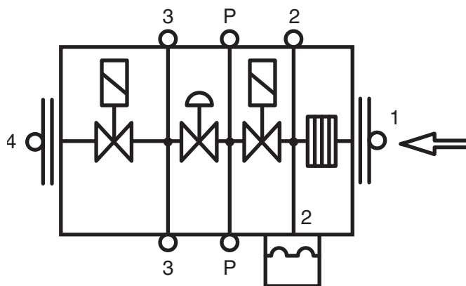
Fig. 16. Pressure tap points for VR415/VR4425/VR420/VR432
