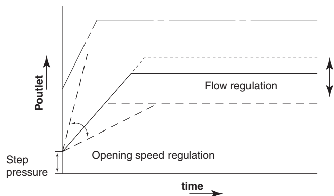
Fig. 15. Characterized opening.
