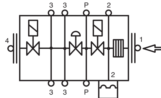
Fig. 17a. Pressure tap points for VR434 only
