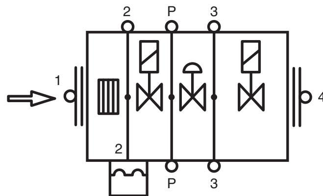
Fig. 17. Pressure tap points for all versions
