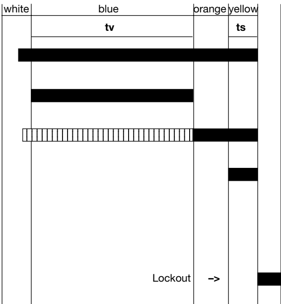
b) Start sequence, flame not established
