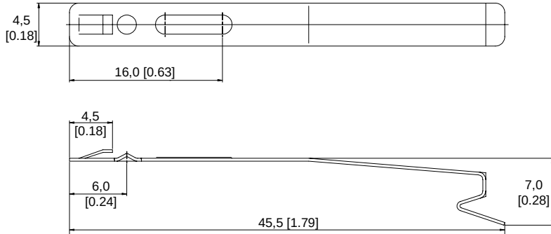
Figure 2. Dimensions
