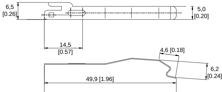
Figure 2. Dimensions
